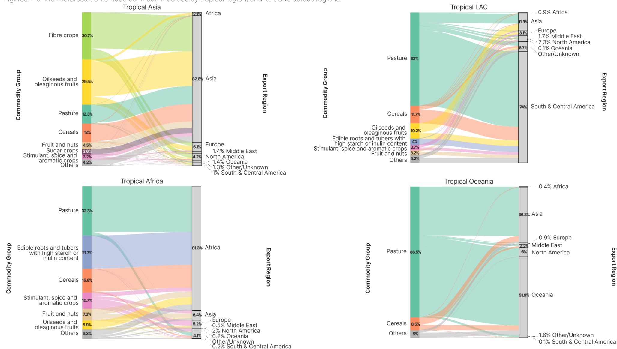
Figures 1.10-1.13. Deforestation embodied in commodities by tropical region, and its trade across regions.
